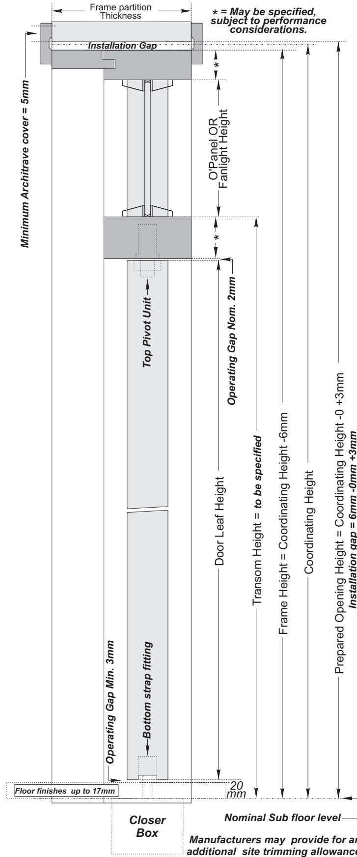
Storey Height Doorset - Double Action - Transomed Over panel OR Glazed Fanlight Option 1
