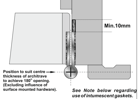
Hinge Specification FD60:
