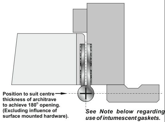
Hinge Specification FD30:
