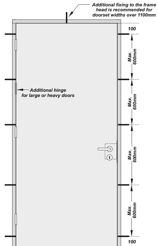
Timber frame fixing locations illustrated.
