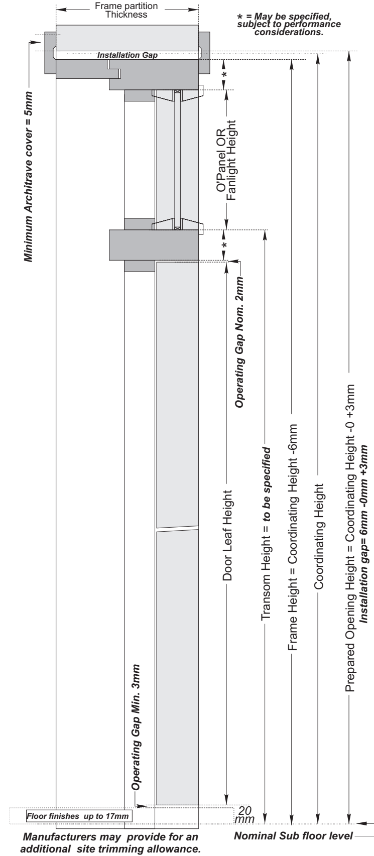
Storey Height Doorset - Single Action - Transomed Over panel OR Glazed Fanlight Fig. 9.12
