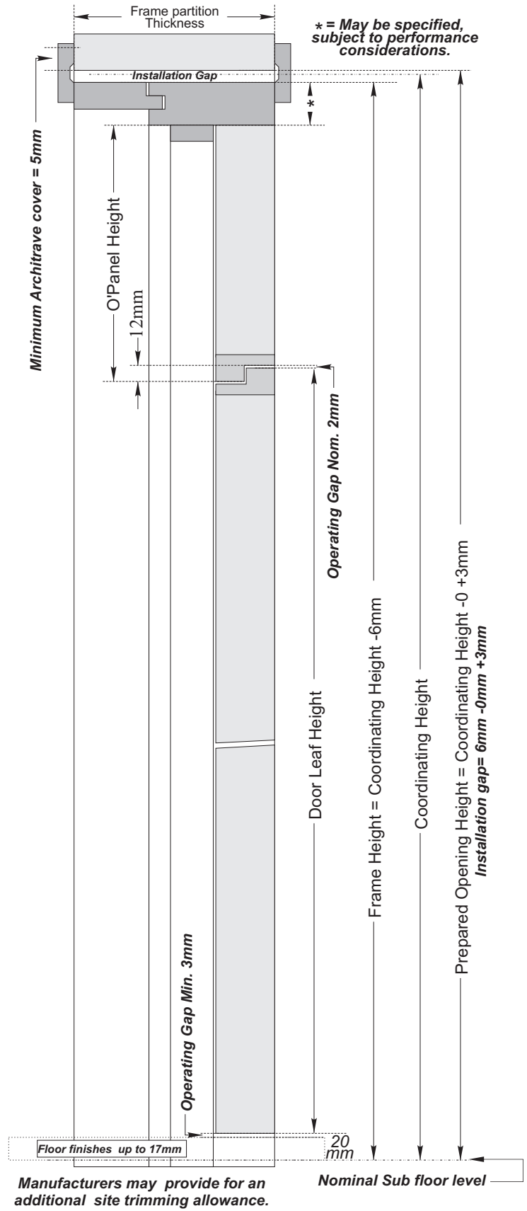
Storey Height Doorset - Single Action - Double Leaf (Pairs) - Flush Over panel Fig. 9.14
