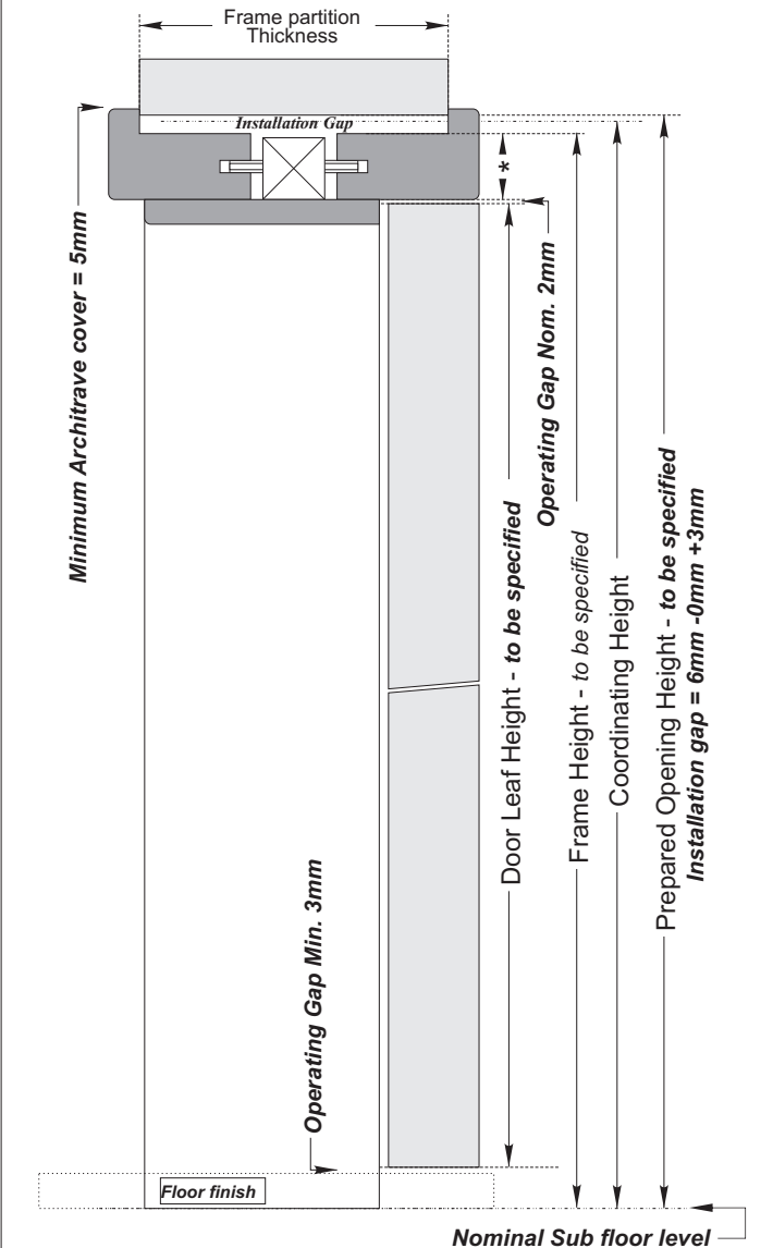
Precision Method - Door Height Doorset - Single Action Fig. 9.27
