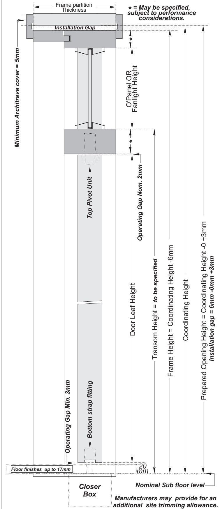
Storey Height Doorset - Double Action - Transomed Over panel OR Glazed Fanlight Option 1 Fig. 9.20
